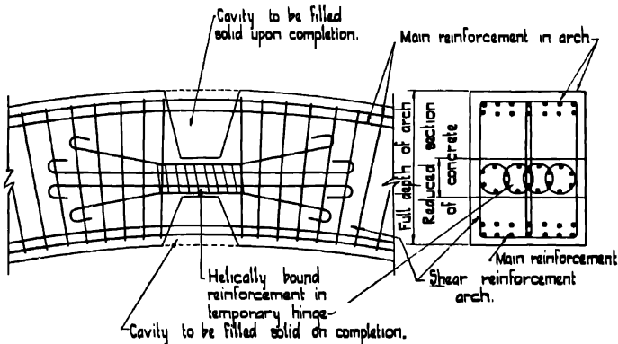
Fig. 334.—Elevation and Section of Temporary Hinge at Crown of Arch Rib.
